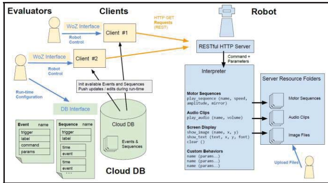
Fig. 2 Architecture of OpenWoZ [13]
